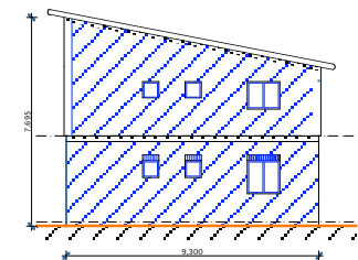
WEST ELEVATION
