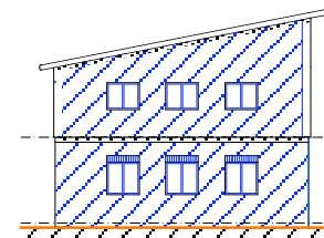
EAST ELEVATION
