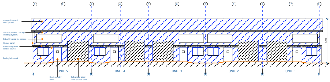
EAST ELEVATION
